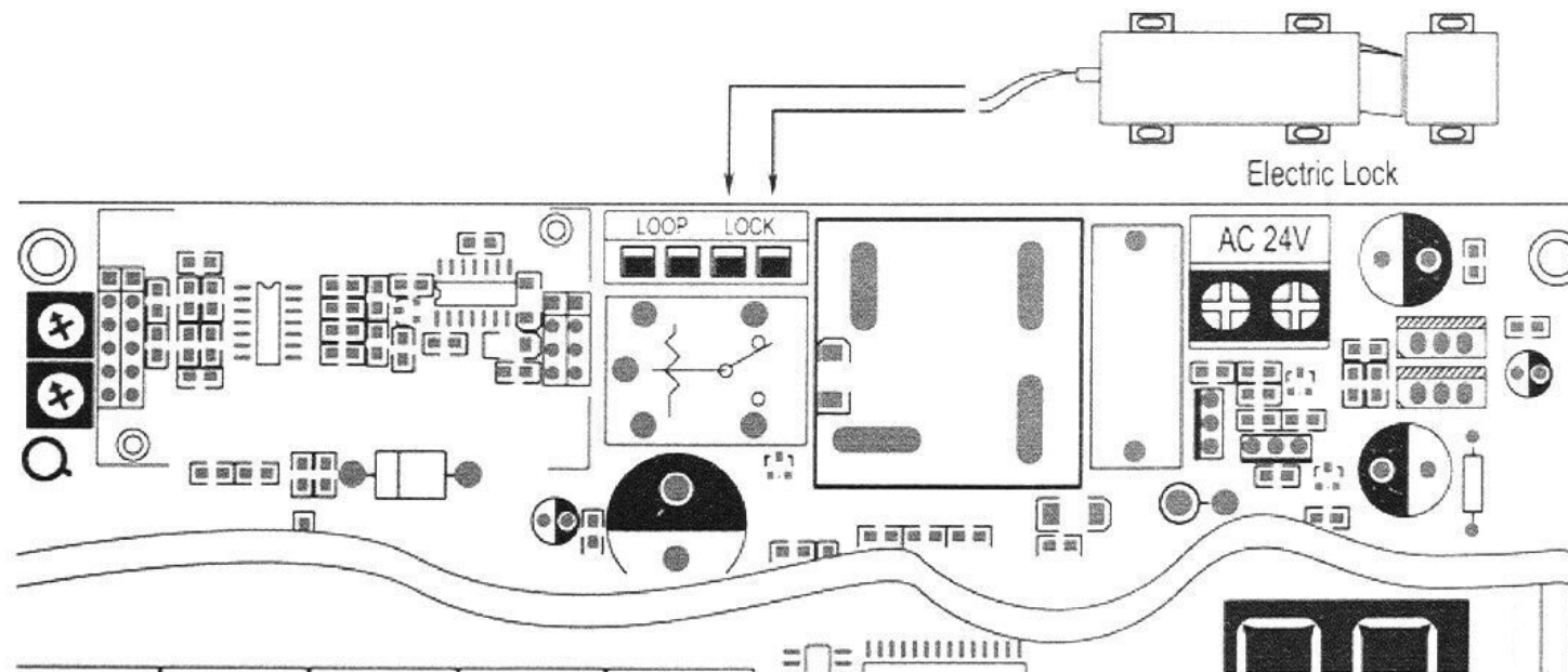
Wiring Diagram of the E-Lock to the MK/LM (KNL 12, 15, 14) Series Swing Gate Opener with electric lock terminal
